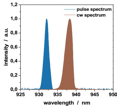
Spectral Characteristic*
