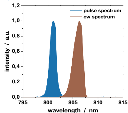
Spectral Characteristic*
